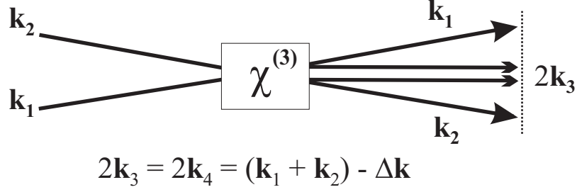
FIG. 1: Wave vector configuration for weak-wave advancement.
